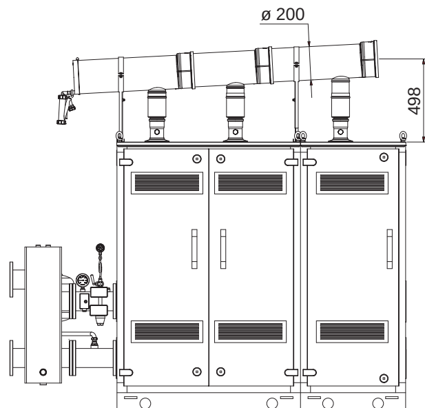
MURELLE EQUIPE 330 BOX ErP exhaust manifold kit code 8102531
