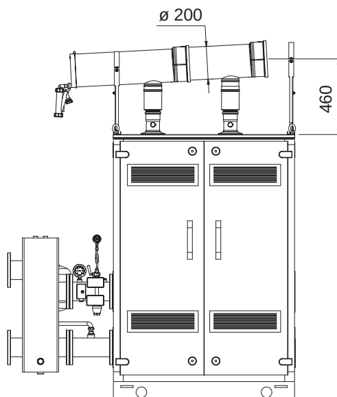
MURELLE EQUIPE 220 BOX ErP exhaust manifold kit code 8102530
